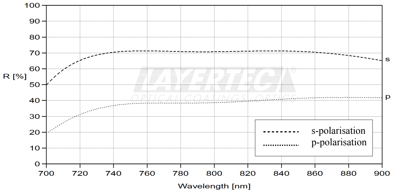
fig. 1 reflection PR-region 45°
