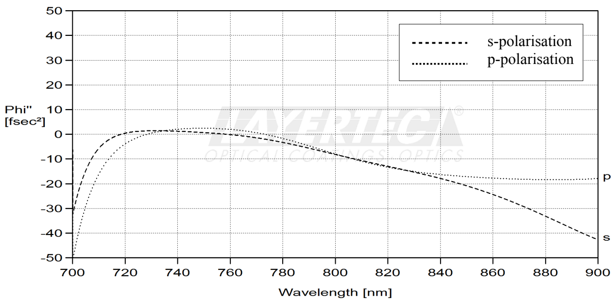
fig. 2 calculated GDD(R, 45°)
