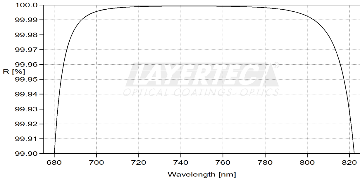
fig. 1 reflection HR-region 0°
