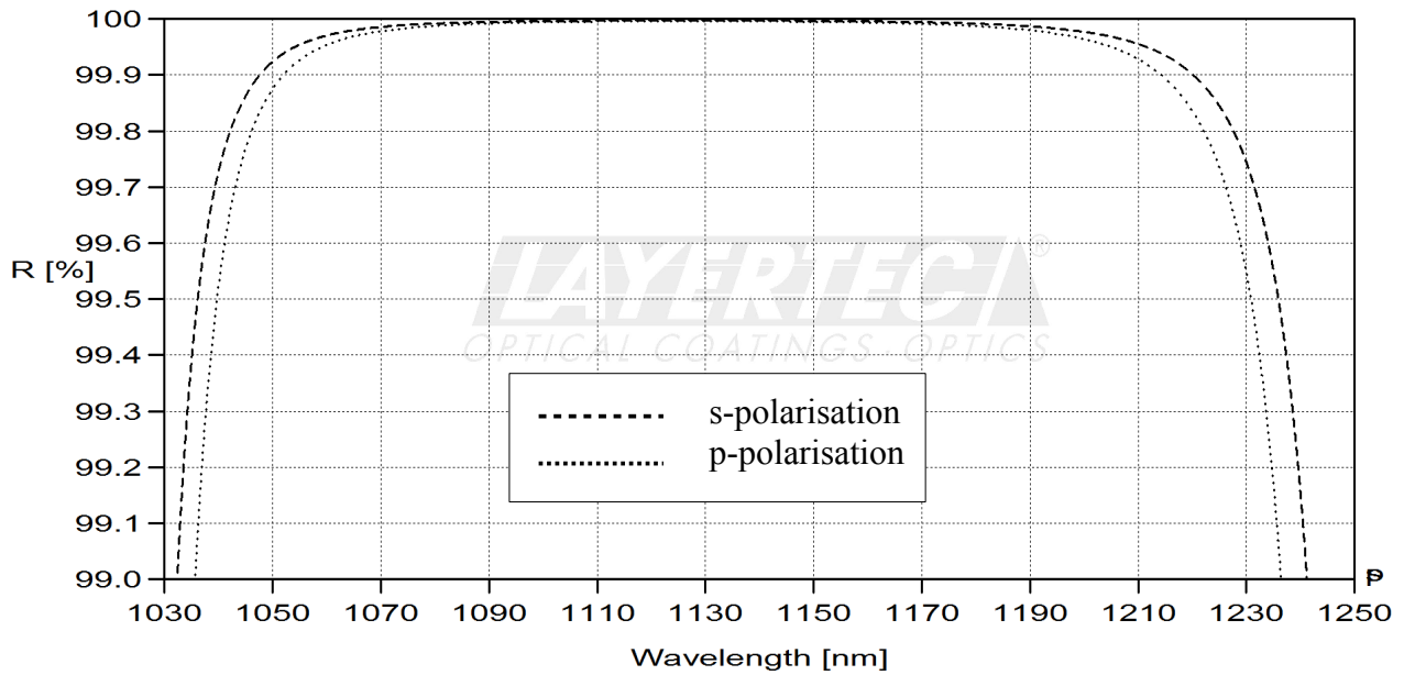
fig. 1 reflection HR-region 12°
