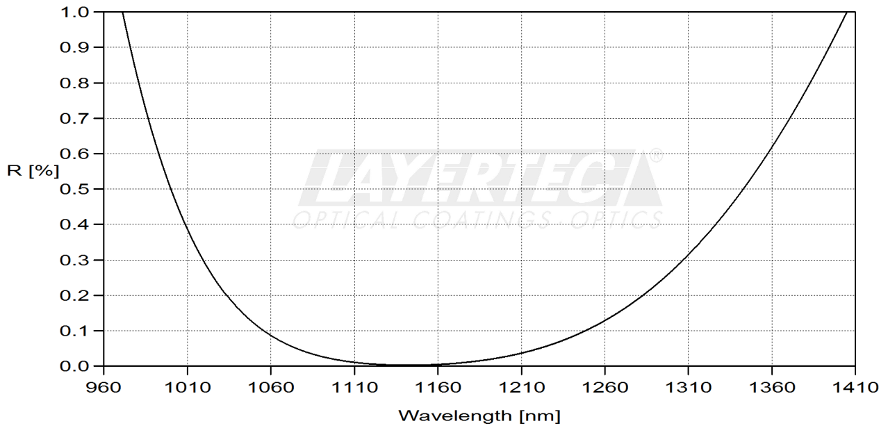
fig. 1 reflection AR 0°
