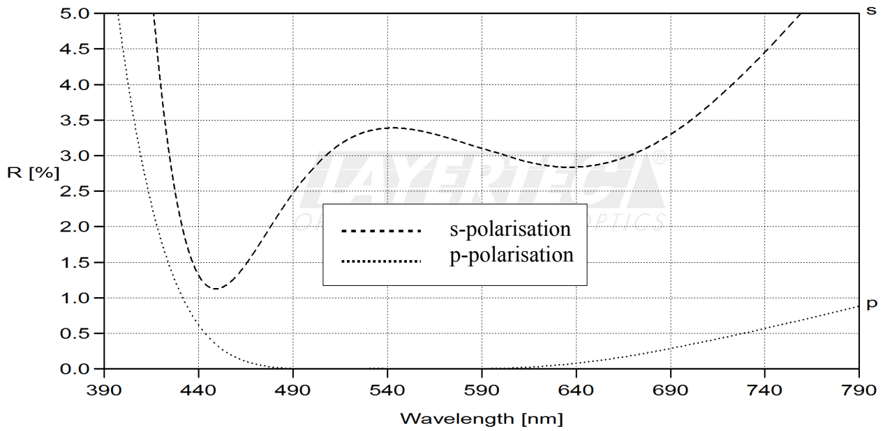
fig. 1 reflection AR 45°
