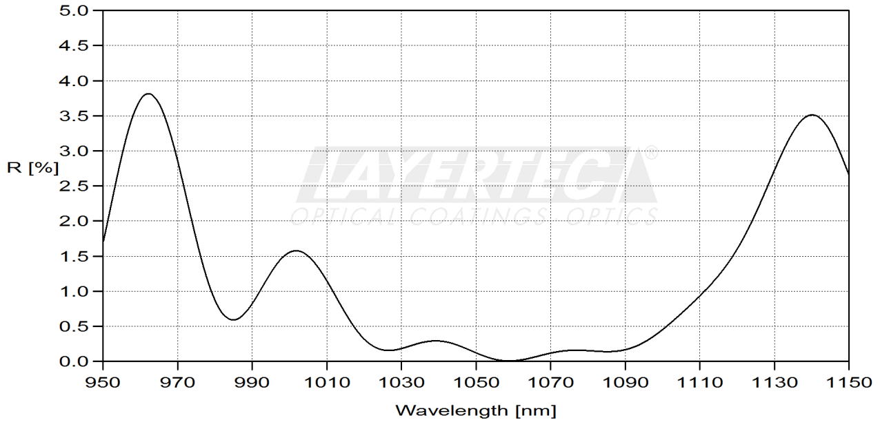
fig. 3 reflection R-region 0°
