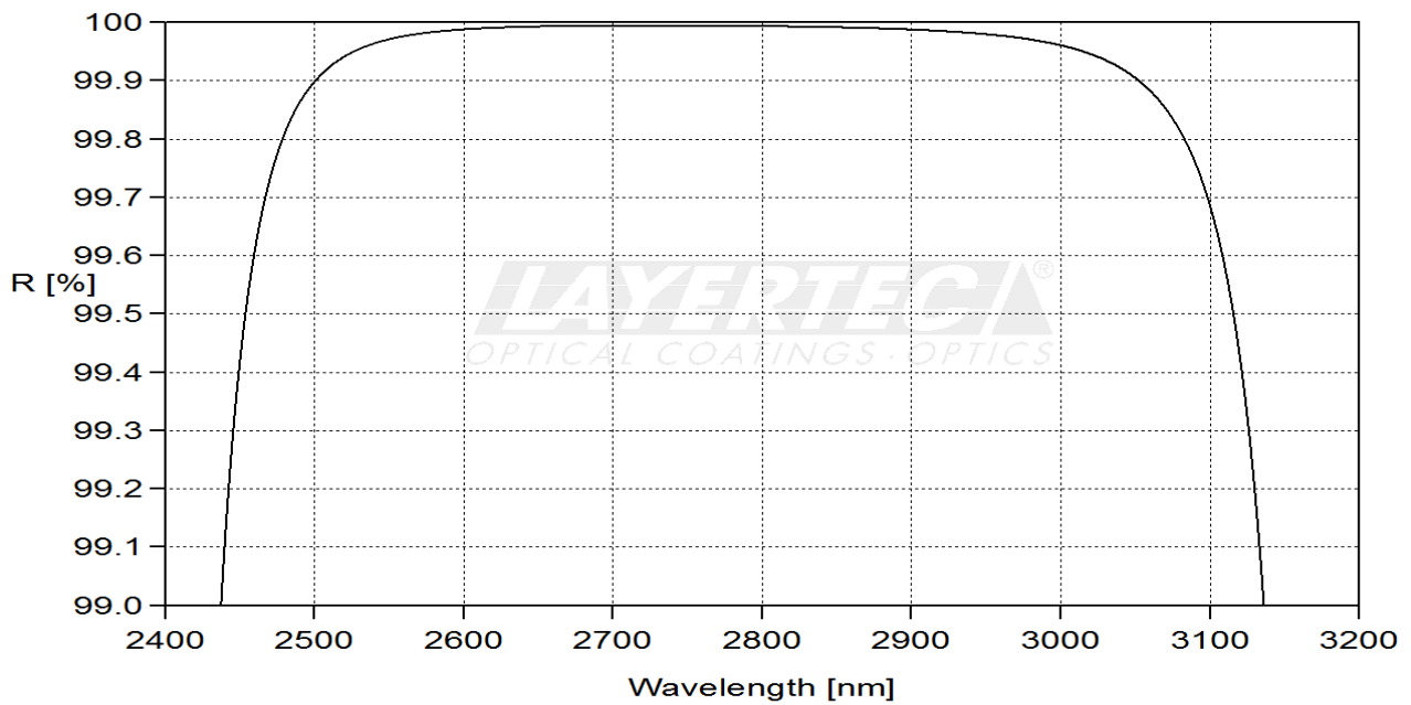
fig. 2 reflection HR-region 0°
