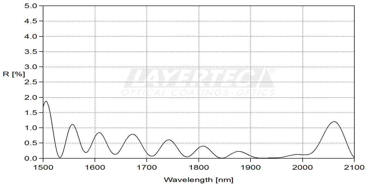
fig. 3 reflection HT-region 0°
