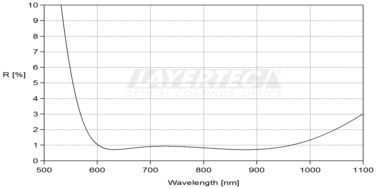
fig. 1 reflection AR 45° (unpolarized)
