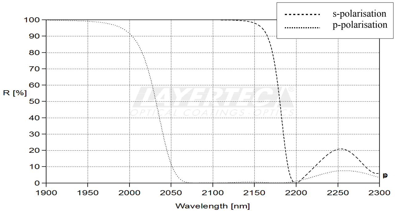
fig. 1 reflection for p- and s-polarisation for AOI=55°
