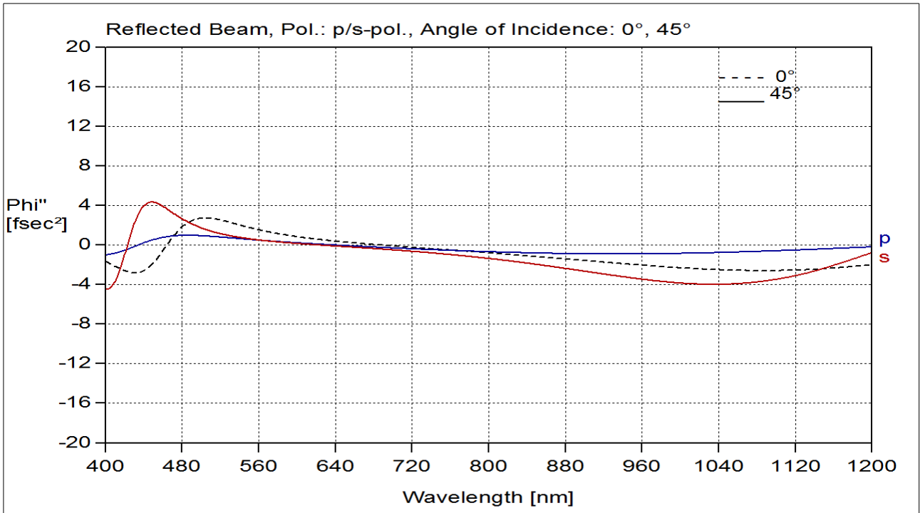
fig. 2 GDD of the reflected beam
