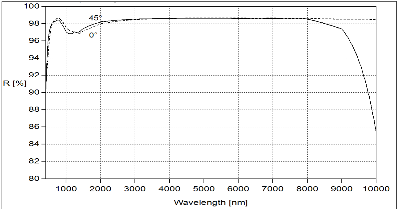
fig. 1 calculated reflectivity 0°, 45°
