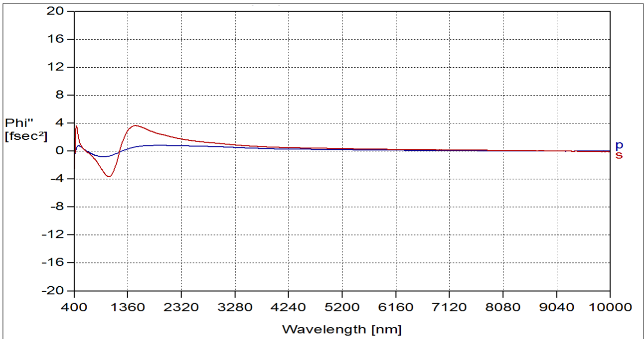
fig. 2 calculated GDD of the reflected beam 45°
